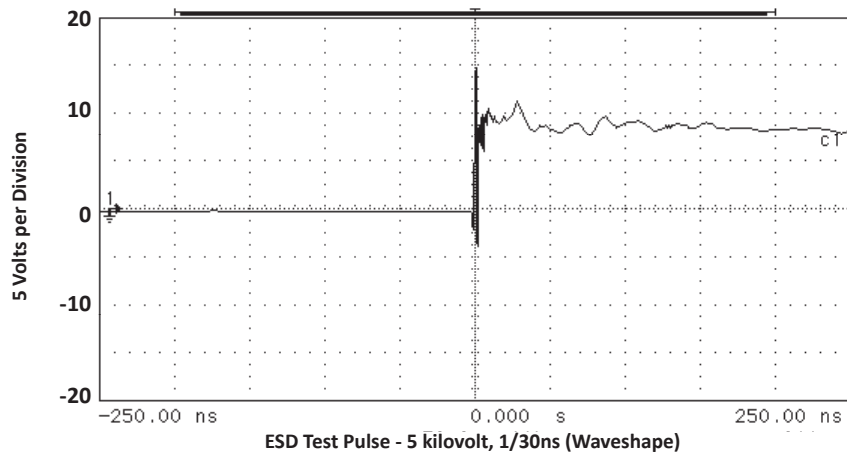
ESD Test Pulse - 5 kilovolt, 1/30ns (Waveshape)
