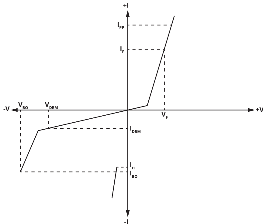
FIGURE 1 VI CHARACTERISITC CURVE
